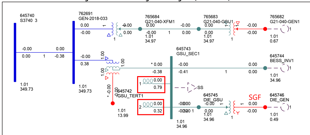
Figure 4: SGF & EGF Single Line Diagram (Shunt Sizes)
