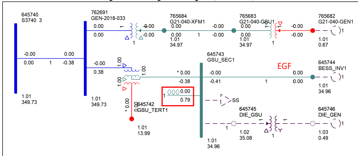
Figure 3: EGF Single Line Diagram (Shunt Sizes)
