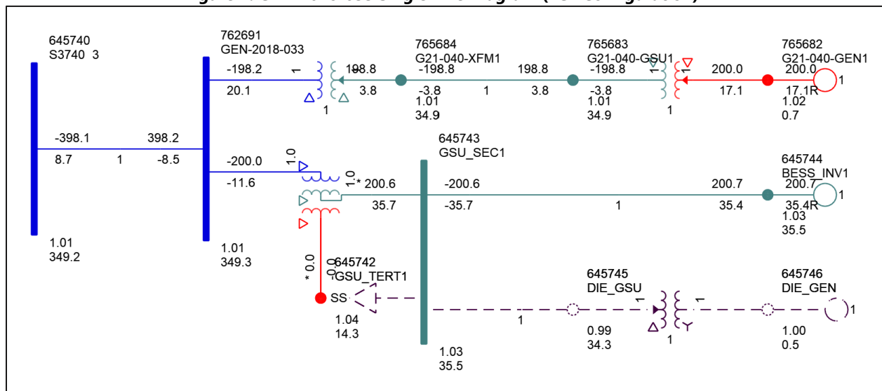
Figure 1: GEN-2018-033 Single Line Diagram (EGF Configuration)
