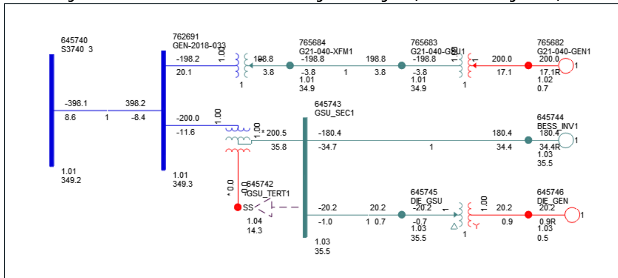
Figure 2: GEN-2018-033 & GEN-2025-SR26 Single Line Diagram (EGF & SGF Configuration)
